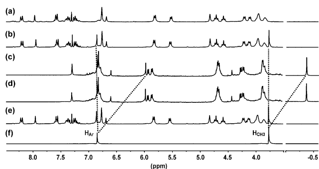
Figure 6. Partial ^1\text{H} NMR spectra (400 MHz, \text{CDCl}_3 ) of a) host 3 b) addition of 1 equiv of 1,4-(MeO) _2 C _6 H _4 into host 3 solution without irradiation, c) 4 \odot 1,4-(MeO) _2 C _6 H _4 , [16] d) c after 4 weeks in dark and RT, e) irradiation of c with light at 254 nm for 1 h or heating at 60 °C for 20 min, f) guest 1,4-(MeO) _2 C _6 H _4 .
